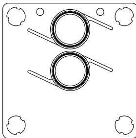
ASSEMBLY P/N: MSA-043-215 INTERFACE SIZE: 1.500" FASTENER SIZE: M5 or 10-32 BOLT PATTERN: 1.188" x 1.188"
