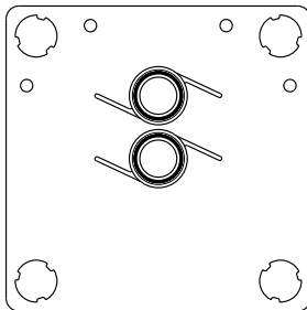
ASSEMBLY P/N: MSA-028-215 INTERFACE SIZE: 1.500" FASTENER SIZE: M5 or 10-32 BOLT PATTERN: 1.188" x 1.188"
