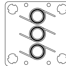
ASSEMBLY P/N: MSA-028-311 INTERFACE SIZE: 1.125" FASTENER SIZE: M4 or 8-32 BOLT PATTERN: .856" x .856"
