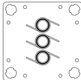
ASSEMBLY P/N: MSA-028-315 INTERFACE SIZE: 1.500" FASTENER SIZE: M5 or 10-32 BOLT PATTERN: 1.188" x 1.188"
