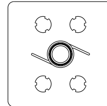
ASSEMBLY P/N: MSA-028-111-U INTERFACE SIZE: 1.125" FASTENER SIZE: M4 or 8-32 BOLT PATTERN: .370" x .630"
