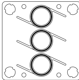
ASSEMBLY P/N: MSA-043-315 INTERFACE SIZE: 1.500" FASTENER SIZE: M5 or 10-32 BOLT PATTERN: 1.188" x 1.188"
